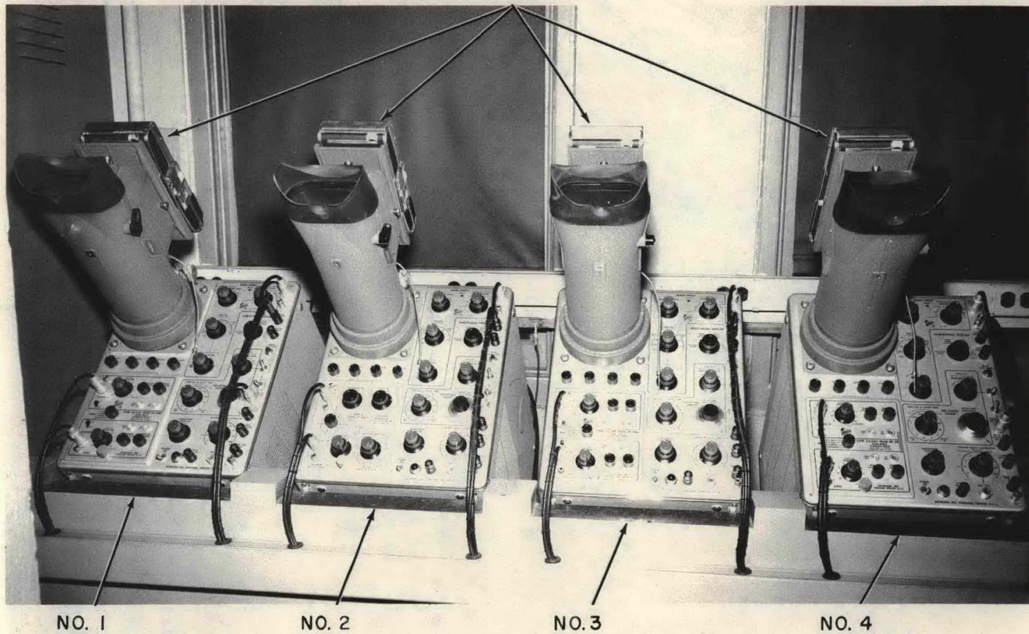
FIG. 2 RECORDING OSCILLOSCOPES
